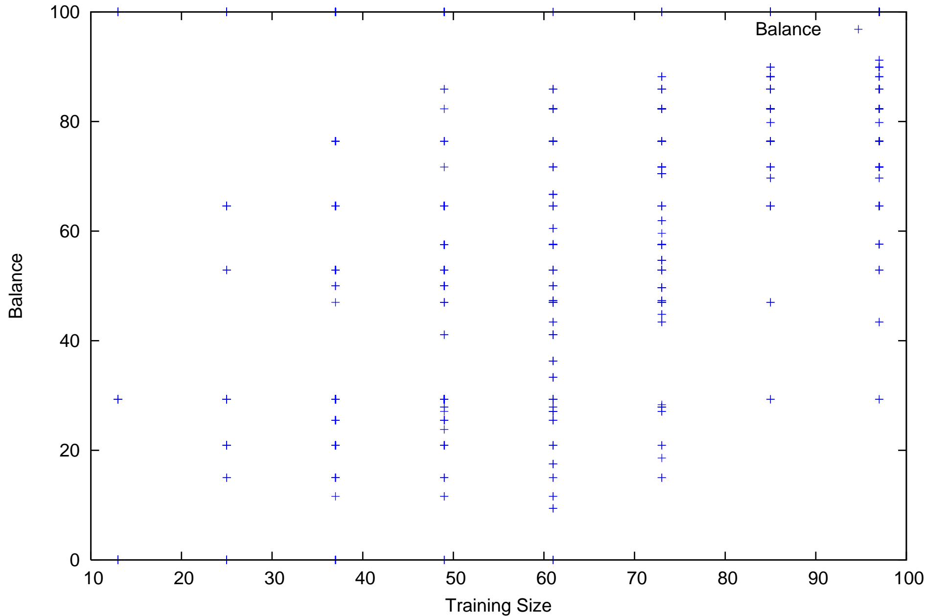
JM1_stats - Component 17 - subsampling
