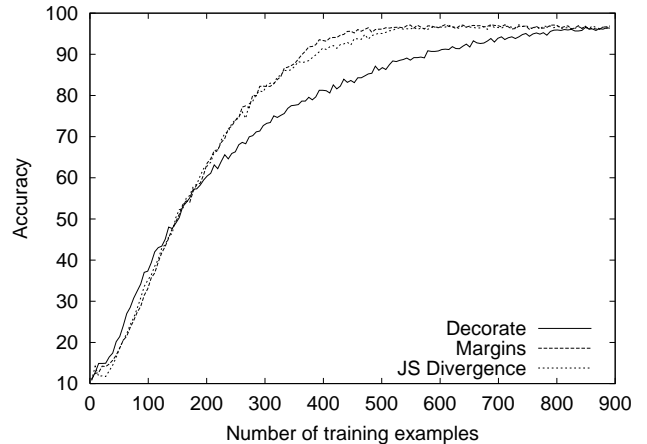
Figure 3. Comparing measures of utility: JS Divergence vs Margins on Vowel .
