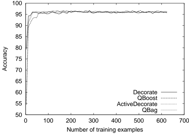
Figure 2. Ceiling effect in learning on Breast-W .
