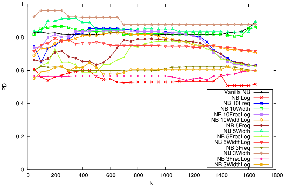
PD for False Class in KC1
