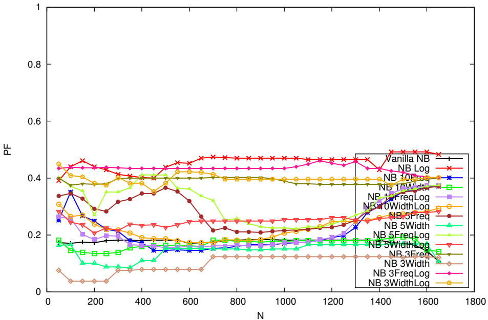
PF for True Class in KC1
