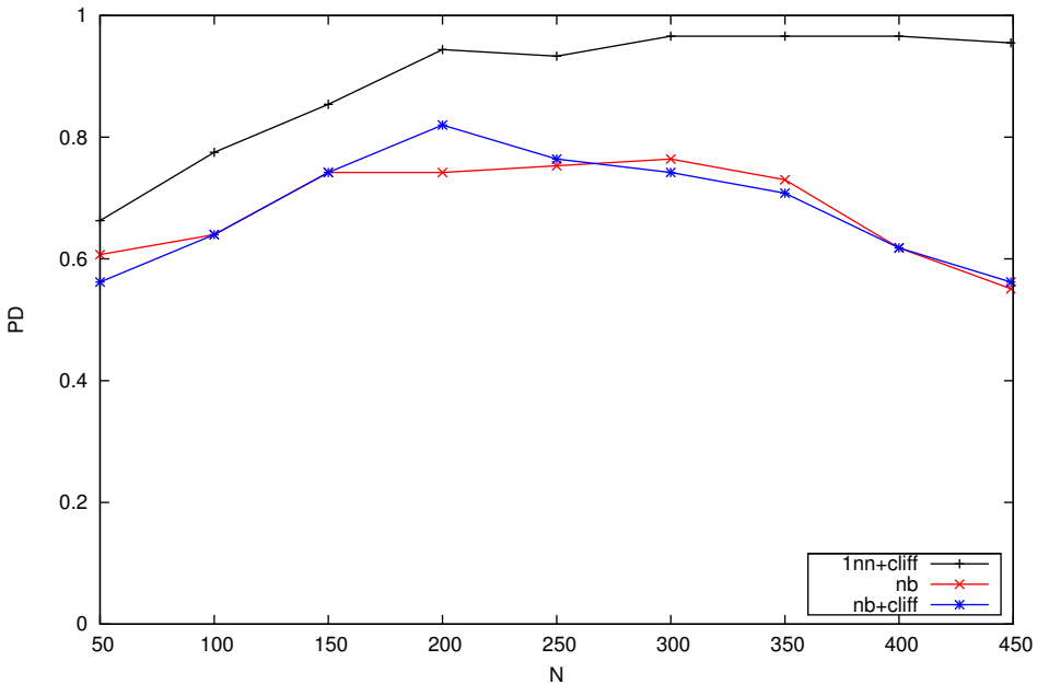
PD for False Class
