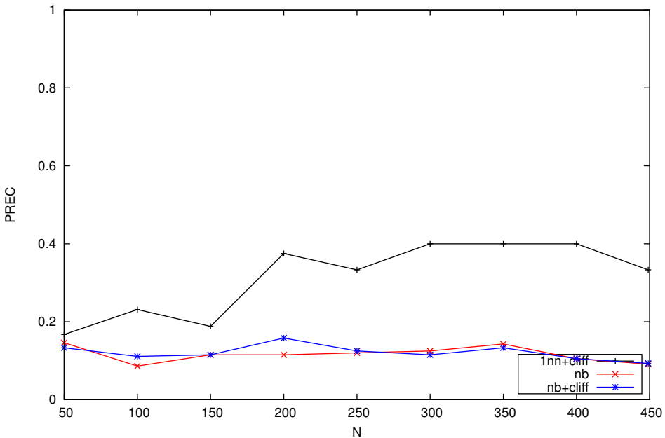
Precision for True Class
